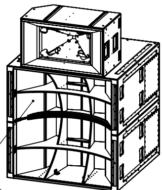
#2) Dimetric View: Two Cabinet Stack: Shown with Interlocking SH96T
