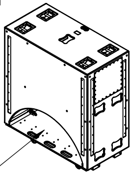
#1) Isometric View: Single Cabinet Positioned for use on Floor or Dolly Board
