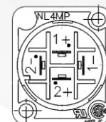
Wiring View of a NL4 Connector
