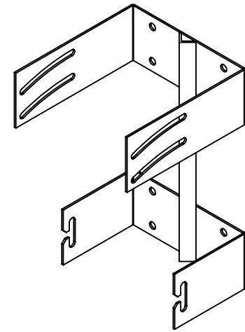
Isometric View: Wall Bracket with 90 Degree Pan Hinge
