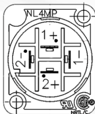
Wiring View of an NL4 Connector
