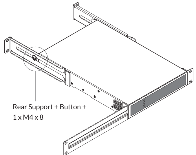
Diagram 3b Danley DSA Rack Support hardware. 2 positions.
